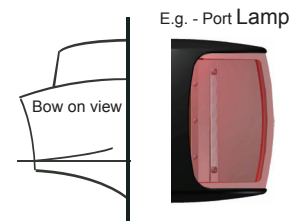
Fig.3 Bi-colour Mounting.
